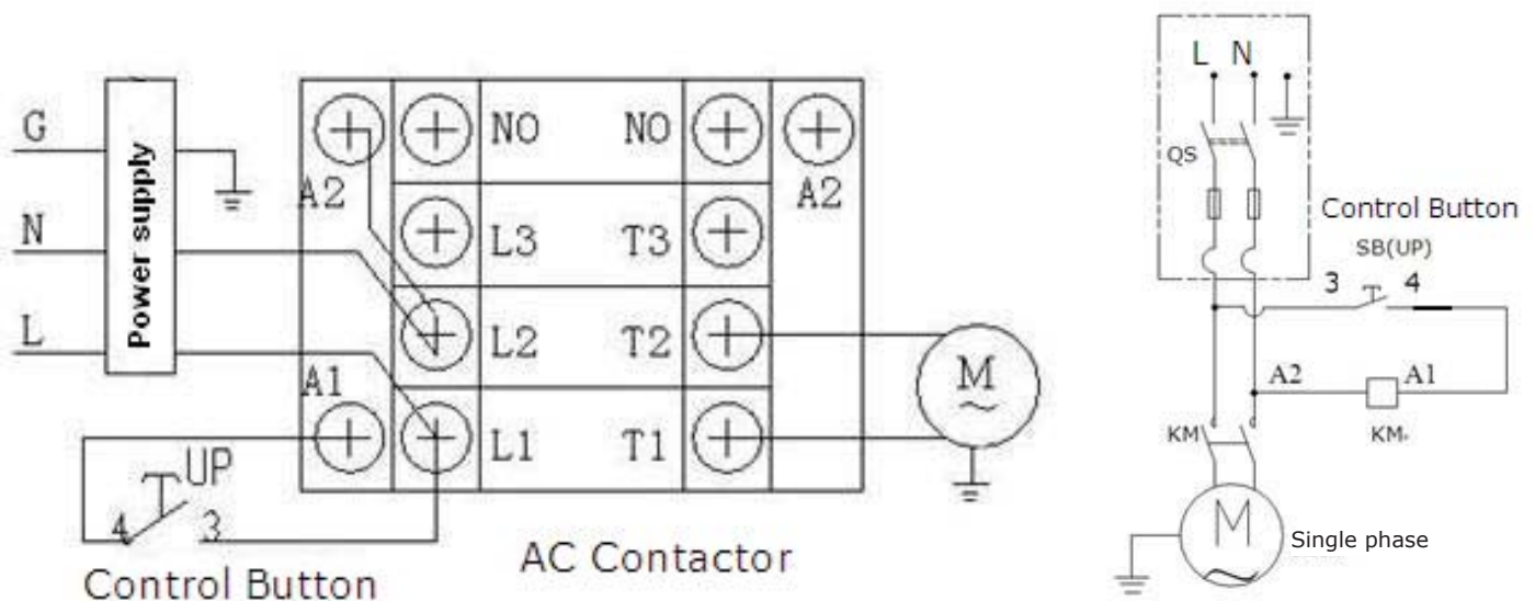
Electric Diagram
